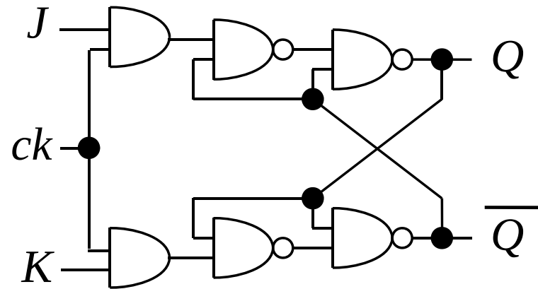
JKFF
