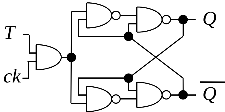
TFF
