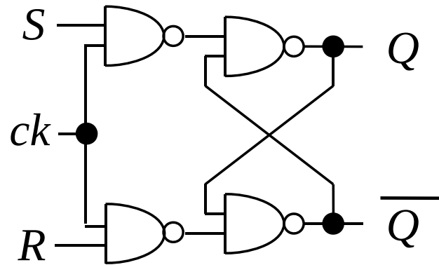
SRFF
